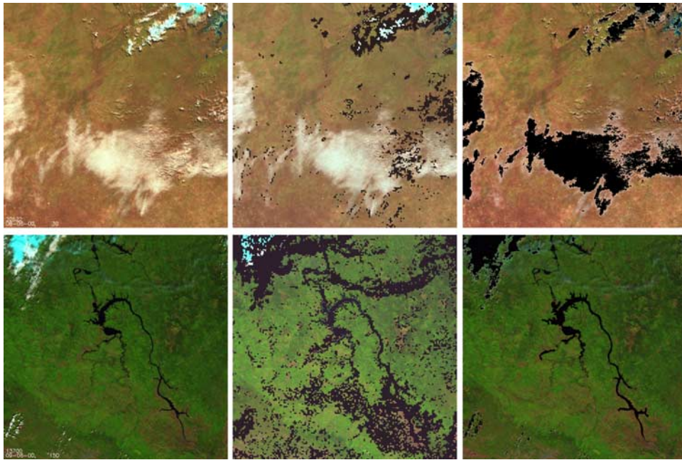
Figure 2. Examples of the new cloud detection scheme over (top panels) Kalahari and (lower panels) Siberia. The images displayed show the (left) original ATSR-2 image, (center) the results obtained from ATSR-2 built-in cloud detection, and (right) the results of the GLOBSCAR cloud detection scheme. Pixels detected as cloudy are shown in black. Water pixels are masked out and for that reason are also shown in black in the image.
