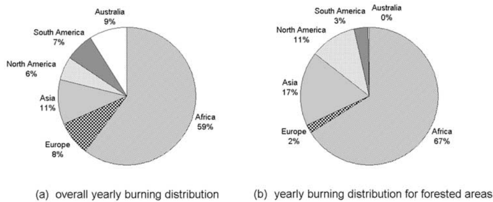
Figure 5. Overall repartition of the burning per continent according to GLOBSCAR results for (a) all vegetated areas and (b) for forested areas only. The biomass burning over Russia is distributed between the European and Asiatic continental figures.
