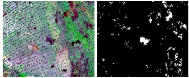
Figure 7. Example of good detection over Mozambique in late August 2000. (left) Some active fires can be seen in the ATSR-2 GBT image. (right) The areas detected as burnt are shown in white.
