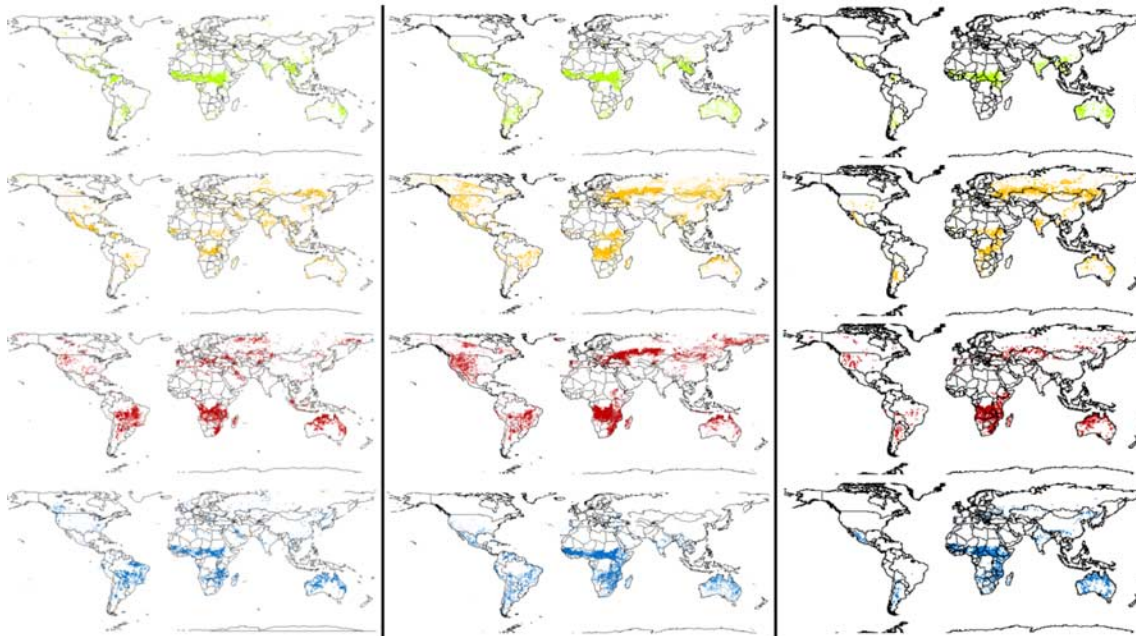
Figure 6. Quick looks of the results obtained by (left) the ATSR world fire atlas, (center) GLOBSCAR, and (right) GBA-2000 results in 2000 presented by 3-month period: January–March, April–June, July–September, and October–December. The GBA-2000 results were visualized using the GBA2000 Web map server hosted at UNEP-GRID ( http://www.grid.unep.ch/activities/earlywarning/preview/ims/gba/ ). The pixel resolution is therefore not exactly the same in the two burnt area products.
