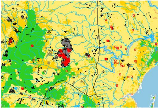
Figure 3. Example of results obtained using the ESA web map server (WMS) over the Kruger National Park, South Africa, in September 2000. The various layers displayed include the IGBP land cover classification, political boundaries and country borders, rivers and lakes (National Imagery and Mapping Agency), ATSR-2 fires (red squares), and GLOBSCAR burnt areas (black polygons with shading).
