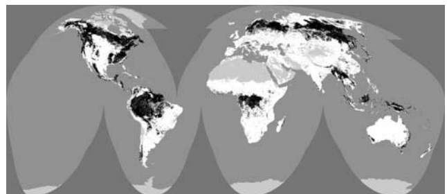
Figure 4. Global distribution of the vegetated areas according to IGBP land cover classification, split into forested (classes 1–5, in black) and nonforested areas (classes 6–12, 14, in white). Nonburnable areas (classes 13, 15–17) are shown by shading.
