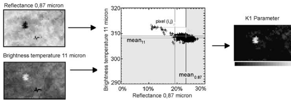
Figure 1. Behavior of burnt surface pixel in the NIR/TIR scatterplot. The pixels that correspond to burned surface move away from the total distribution in the upper left direction. This is due to the increase in temperature and decrease in the NIR reflectance.
