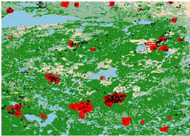
Figure 8. Example of detection of older burnt areas in Canada. Active fires (WFA) from summer 1998 are overlaid with GLOBSCAR results of June 2000 (in black). The area displayed is in the northern part of Canada, around 107^{\circ} west/ 57^{\circ} north.
