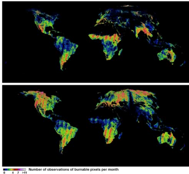
Figure 10. Examples of the number of cloud-free observations available per month using ATSR-2 daytime data, for burnable pixels only. Nonburnable regions (according to IGBP classification) are directly eliminated and therefore shown in black (e.g., water pixels or Sahara region). The highest revisit frequency is at the high latitudes in the summer months. The data gap in Siberia can be seen on the July 2000 picture. The frequent cloud coverage over Indonesia is also clearly shown in these examples.
